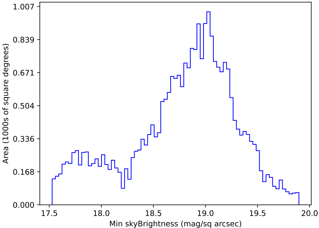
too_elab_r64_d3_gz_v3.4_10yrs Yr 1 i band: Min skyBrightness
