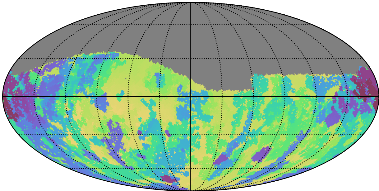
too_elab_r64_d3_gz_v3.4_10yrs Yr 1 g band: Min skyBrightness
