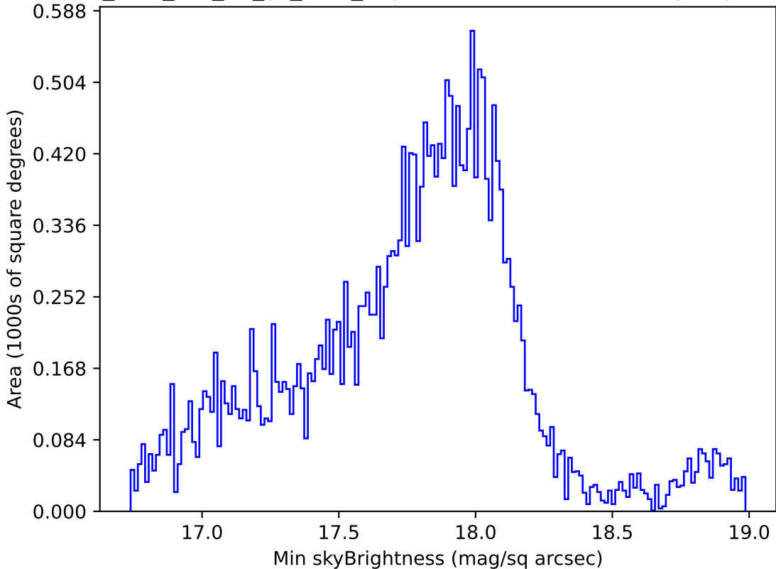
too_elab_r64_d3_gz_v3.4_10yrs Yr 1 all bands: Min skyBrightness
