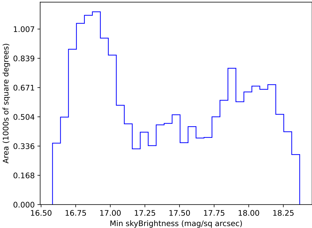
too_elab_r64_d3_gz_v3.4_10yrs WFD z band: Min skyBrightness
