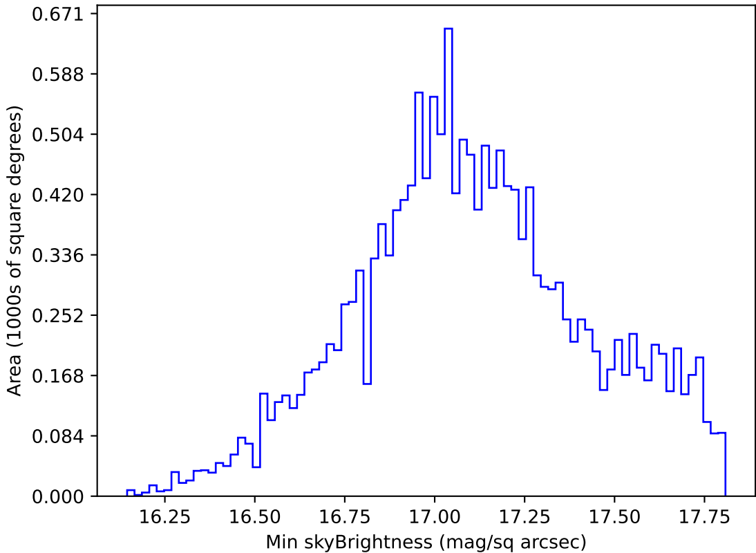
too_elab_r64_d3_gz_v3.4_10yrs WFD y band: Min skyBrightness
