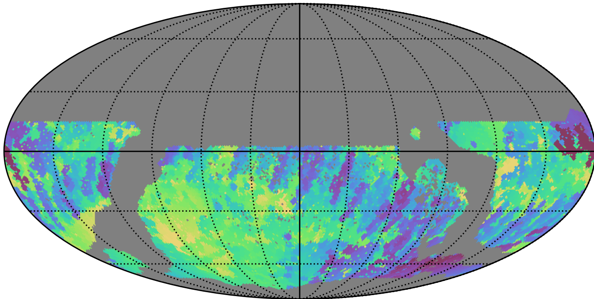
too_elab_r64_d3_gz_v3.4_10yrs WFD r band: Min skyBrightness
