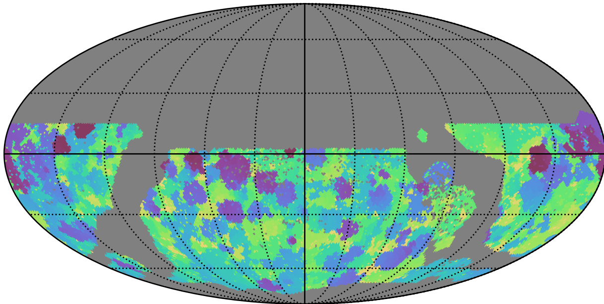
too_elab_r64_d3_gz_v3.4_10yrs WFD g band: Min skyBrightness
