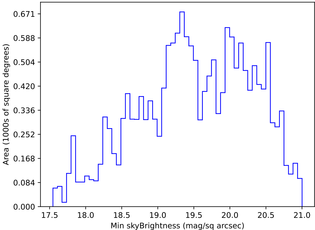
too_elab_r64_d3_gz_v3.4_10yrs WFD g band: Min skyBrightness
