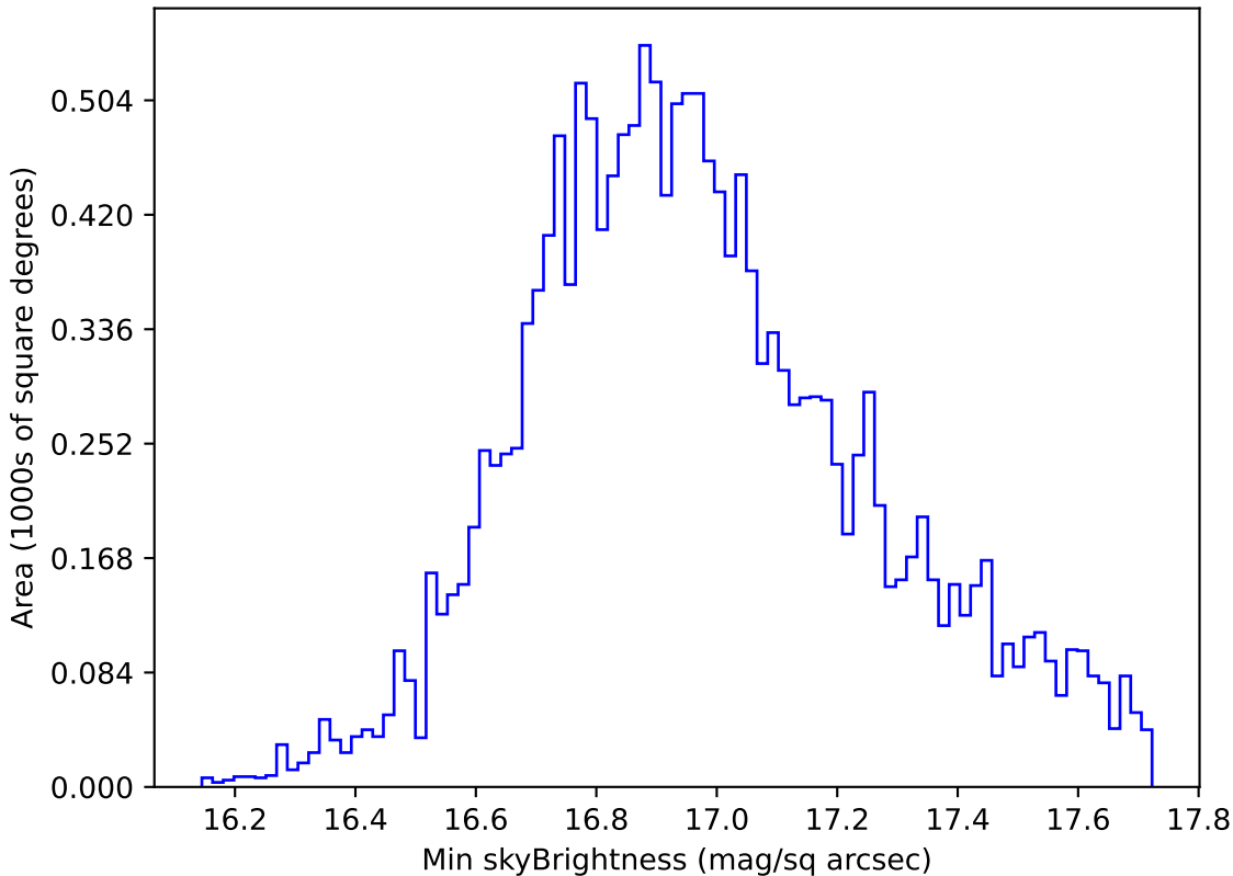
too_elab_r64_d3_gz_v3.4_10yrs WFD all bands: Min skyBrightness
