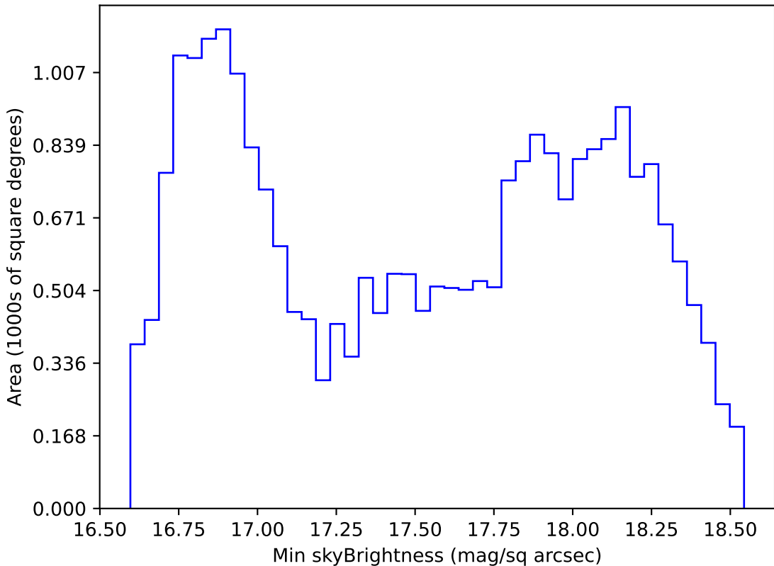
too_elab_r64_d3_gz_v3.4_10yrs All sky z band: Min skyBrightness
