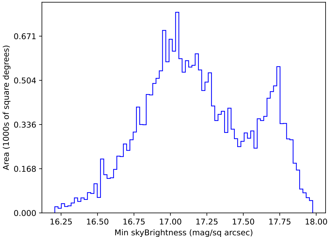
too_elab_r64_d3_gz_v3.4_10yrs All sky y band: Min skyBrightness
