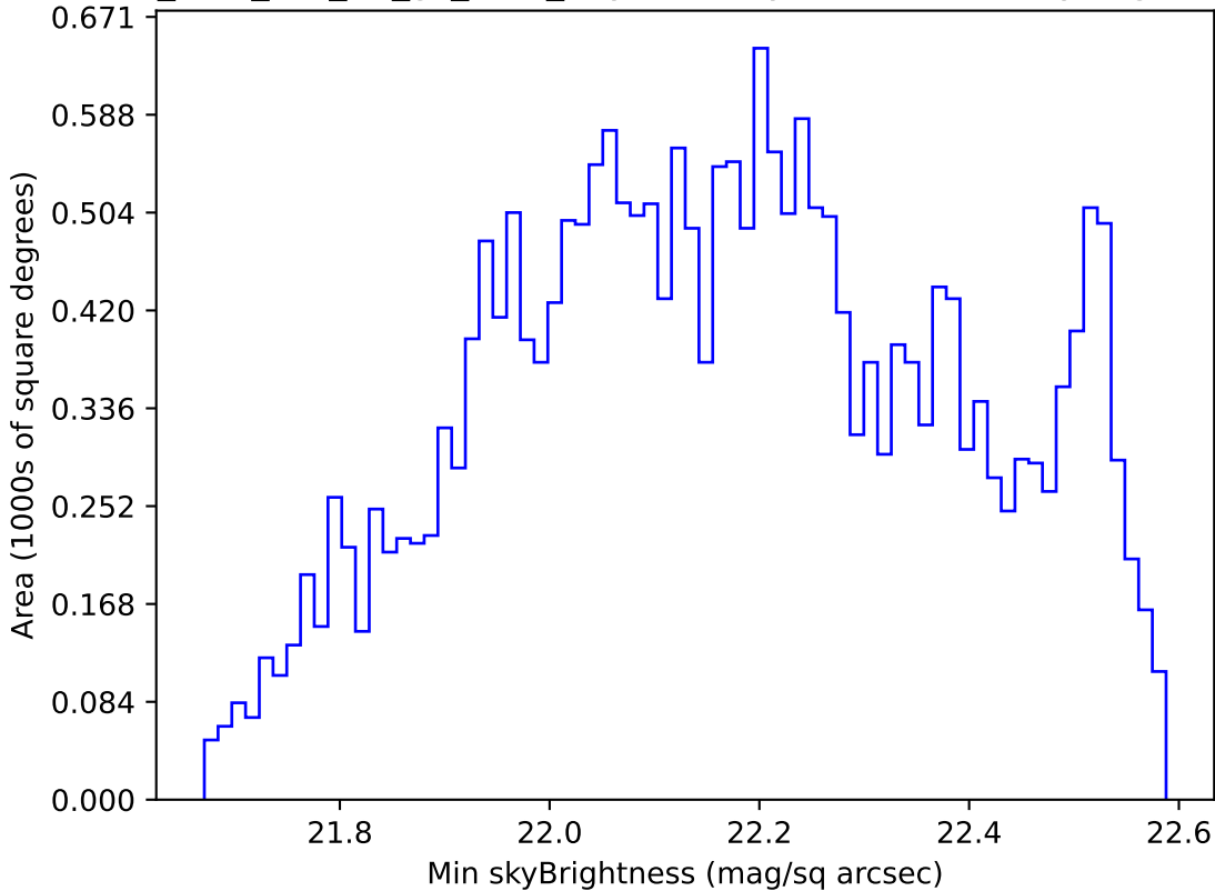
too_elab_r64_d3_gz_v3.4_10yrs All sky u band: Min skyBrightness
