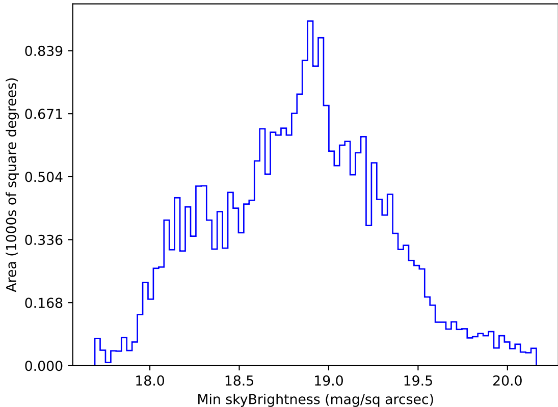
too_elab_r64_d3_gz_v3.4_10yrs All sky r band: Min skyBrightness
