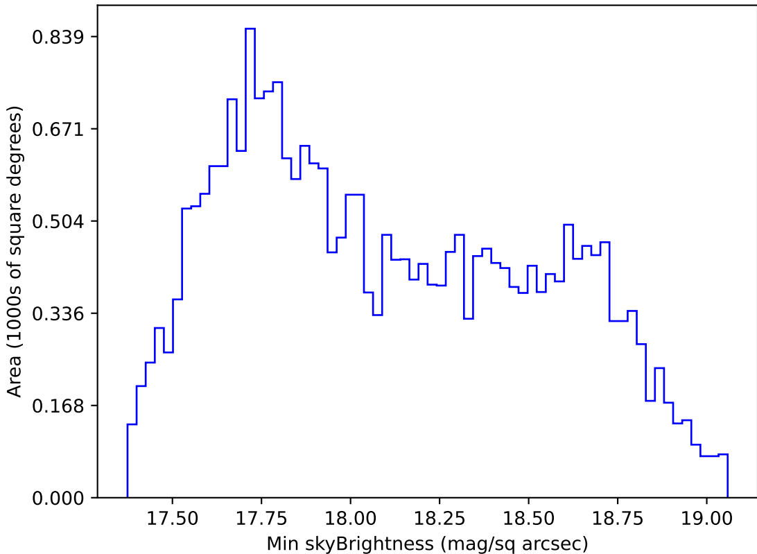
too_elab_r64_d3_gz_v3.4_10yrs All sky i band: Min skyBrightness
