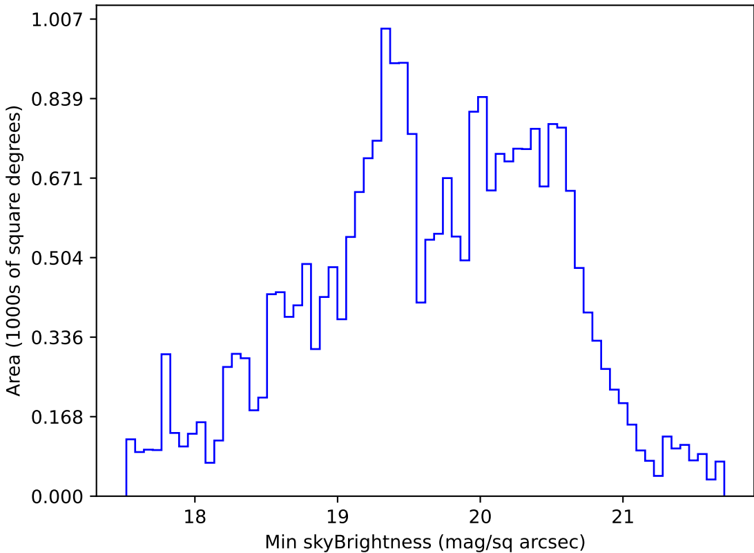
too_elab_r64_d3_gz_v3.4_10yrs All sky g band: Min skyBrightness
