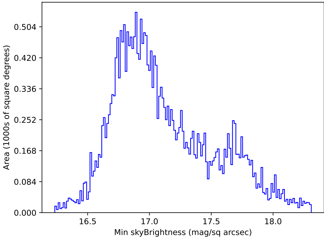
too_elab_r64_d3_gz_v3.4_10yrs All sky all bands: Min skyBrightness
