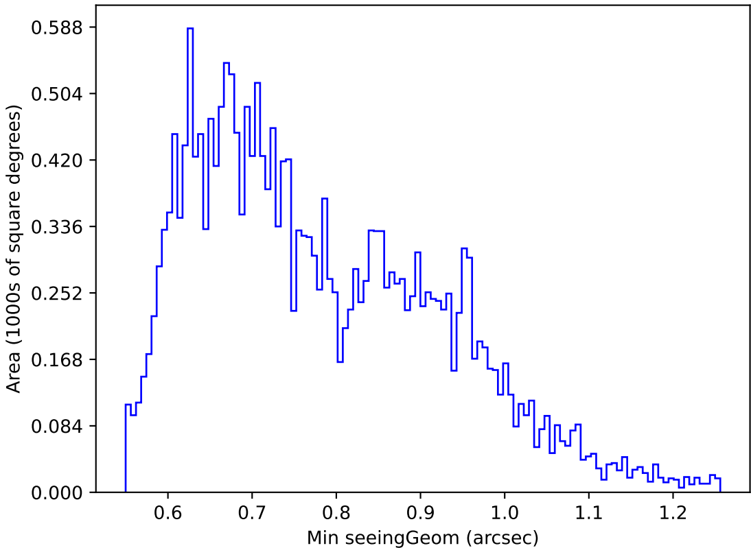
too_elab_r64_d3_gz_v3.4_10yrs Yr 1 u band: Min seeingGeom
