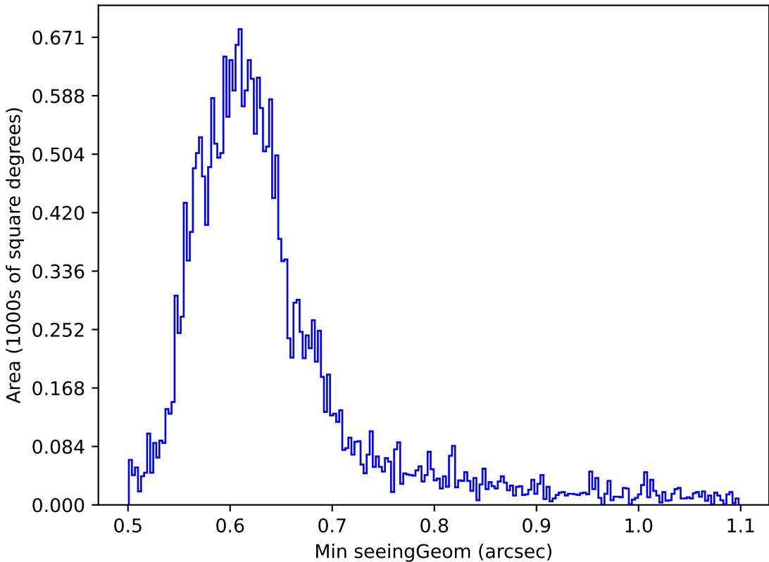
too_elab_r64_d3_gz_v3.4_10yrs Yr 1 r band: Min seeingGeom
