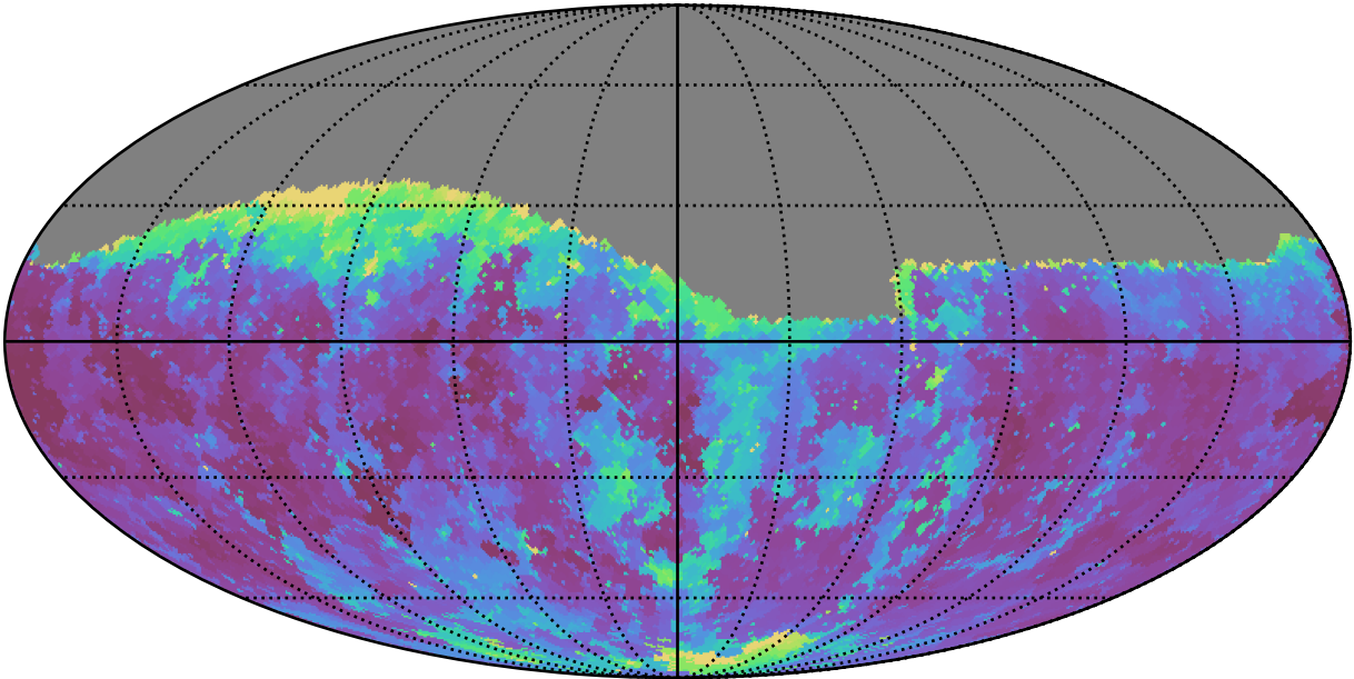
too_elab_r64_d3_gz_v3.4_10yrs Yr 1 g band: Min seeingGeom
