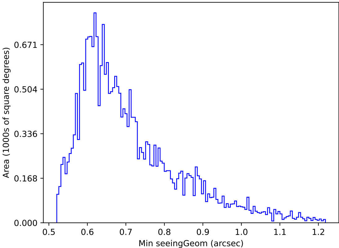
too_elab_r64_d3_gz_v3.4_10yrs Yr 1 g band: Min seeingGeom
