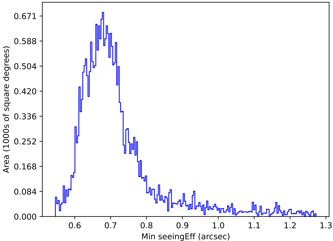
too_elab_r64_d3_gz_v3.4_10yrs Yr 1 r band: Min seeingEff
