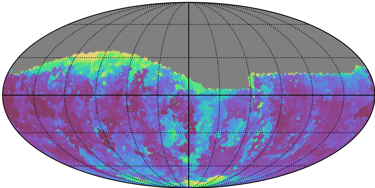
too_elab_r64_d3_gz_v3.4_10yrs Yr 1 g band: Min seeingEff
