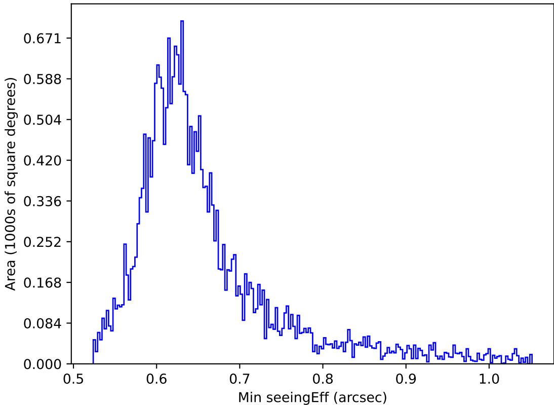
too_elab_r64_d3_gz_v3.4_10yrs Yr 1 all bands: Min seeingEff
