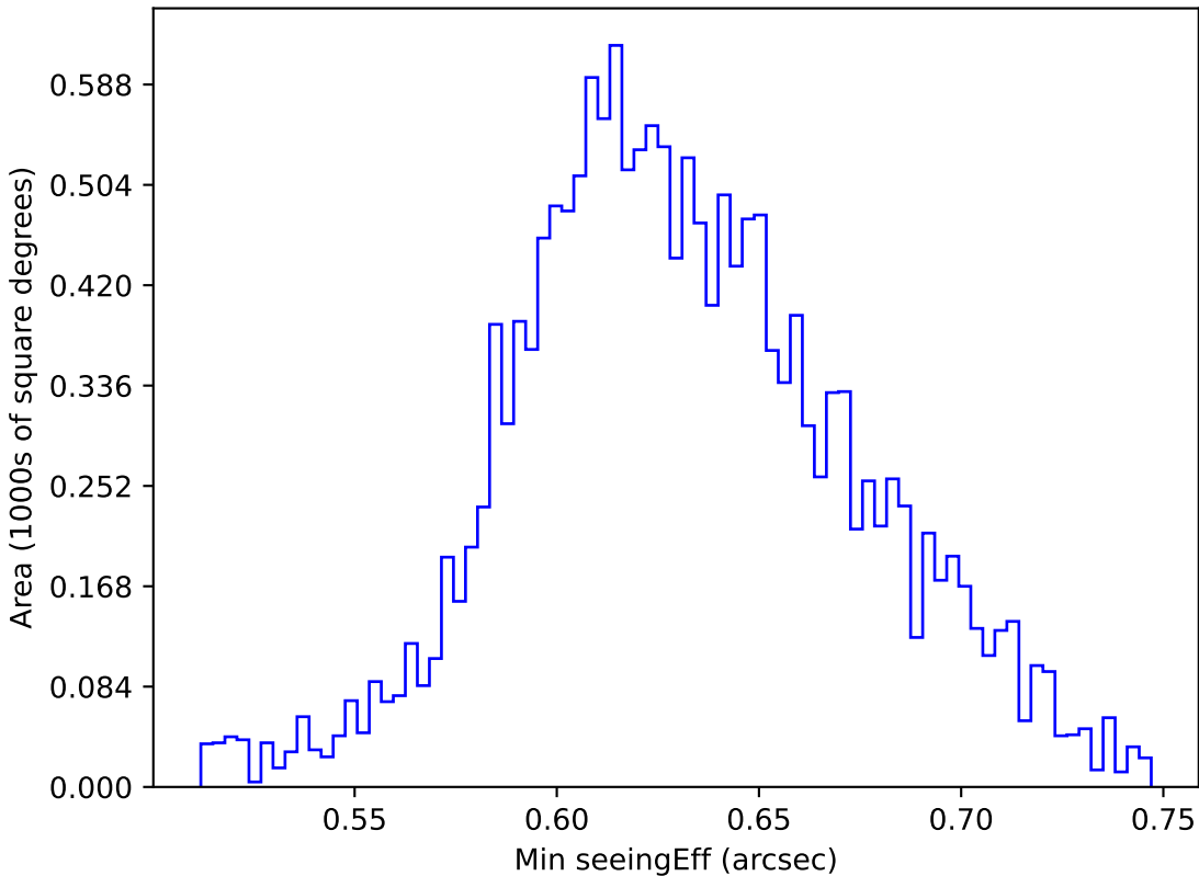
too_elab_r64_d3_gz_v3.4_10yrs WFD y band: Min seeingEff
