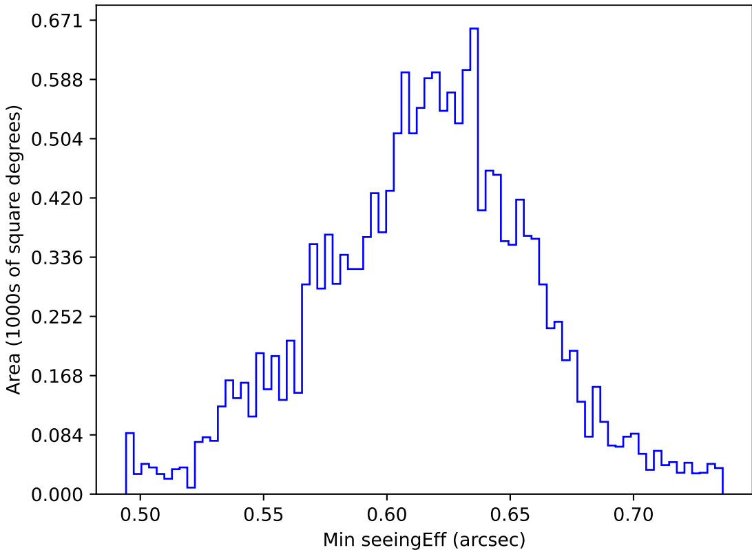
too_elab_r64_d3_gz_v3.4_10yrs WFD r band: Min seeingEff
