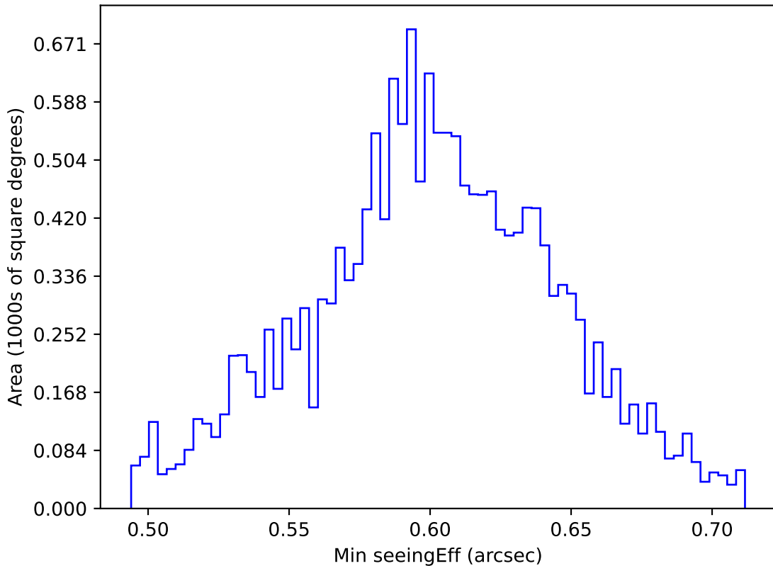
too_elab_r64_d3_gz_v3.4_10yrs WFD i band: Min seeingEff
