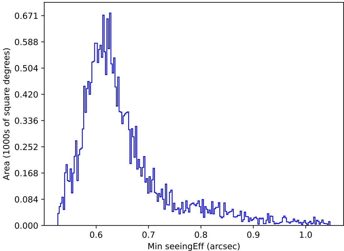
too_elab_r64_d3_gz_v3.4_10yrs All sky z band: Min seeingEff
