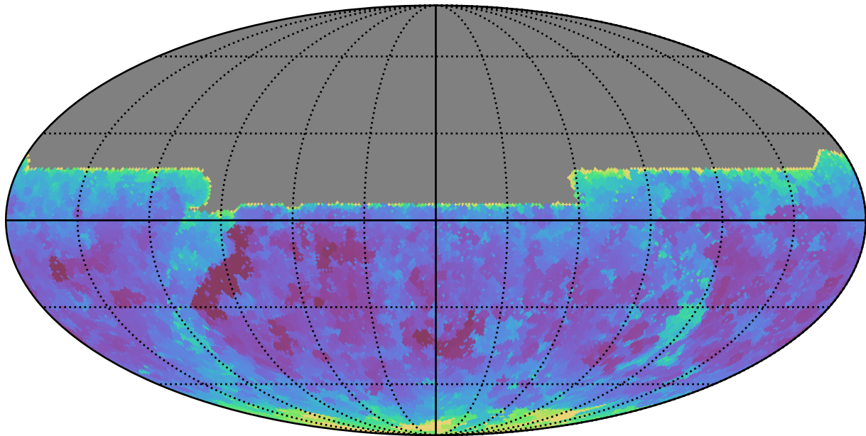
too_elab_r64_d3_gz_v3.4_10yrs All sky y band: Min seeingEff
