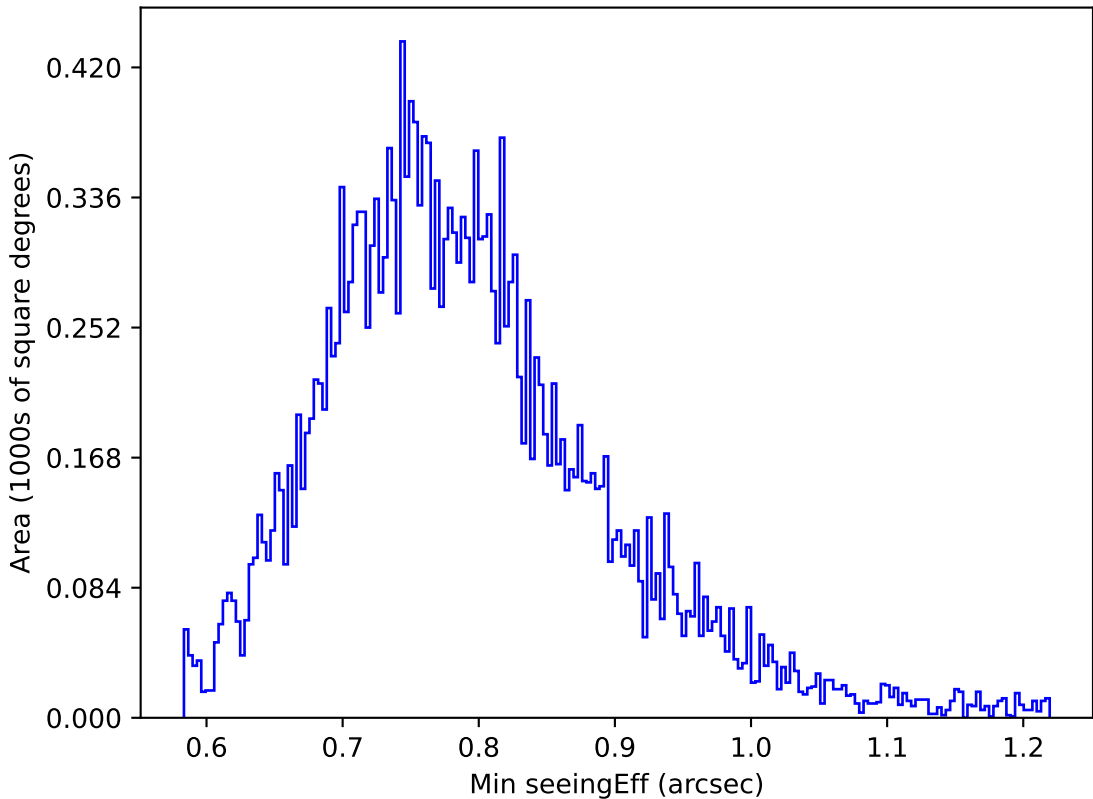
too_elab_r64_d3_gz_v3.4_10yrs All sky u band: Min seeingEff
