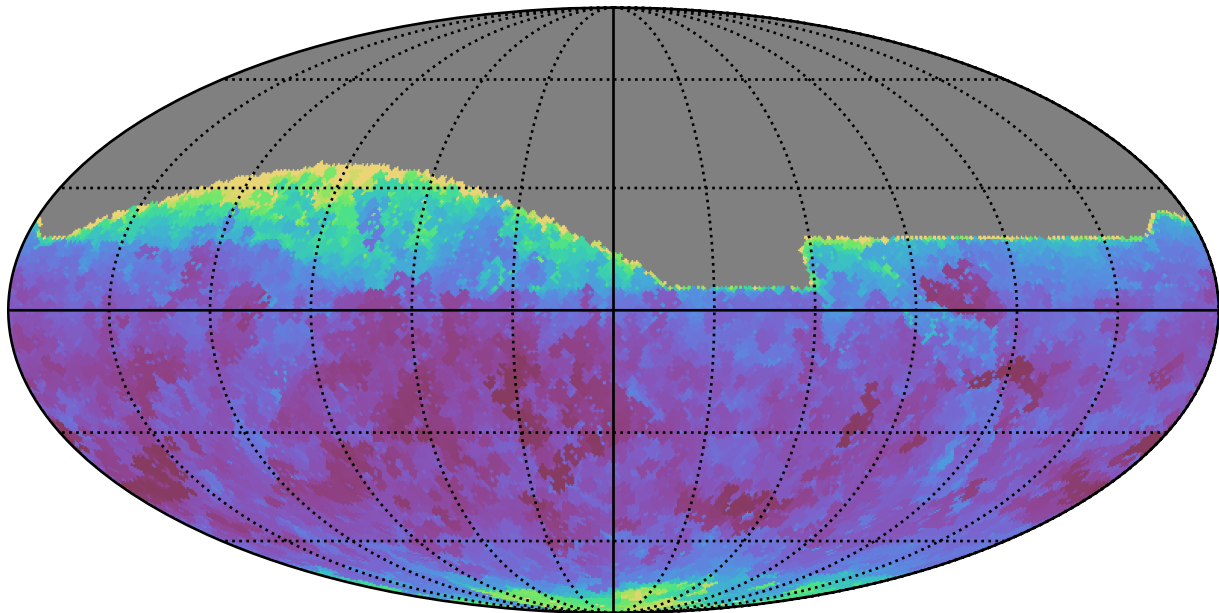
too_elab_r64_d3_gz_v3.4_10yrs All sky i band: Min seeingEff
