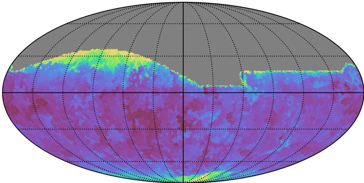
too_elab_r64_d3_gz_v3.4_10yrs All sky g band: Min seeingEff
