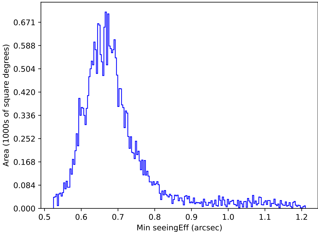
too_elab_r64_d3_gz_v3.4_10yrs All sky g band: Min seeingEff
