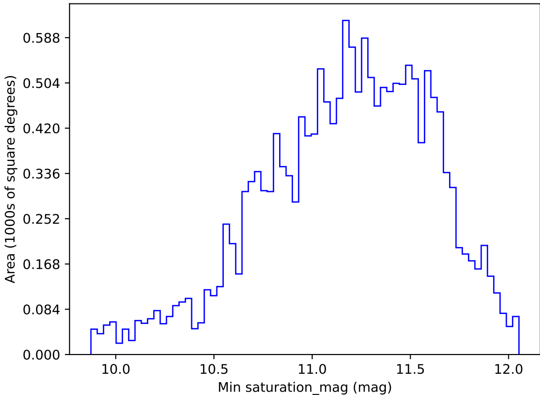
too_elab_r64_d3_gz_v3.4_10yrs WFD y band: Min saturation_mag
