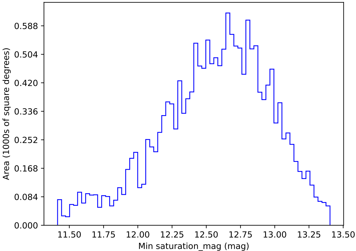
too_elab_r64_d3_gz_v3.4_10yrs WFD r band: Min saturation_mag
