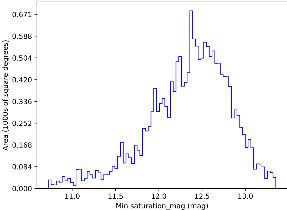
too_elab_r64_d3_gz_v3.4_10yrs WFD i band: Min saturation_mag
