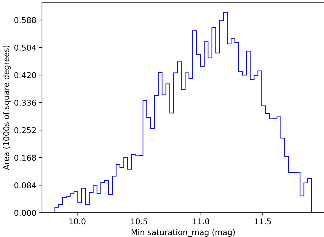
too_elab_r64_d3_gz_v3.4_10yrs WFD all bands: Min saturation_mag
