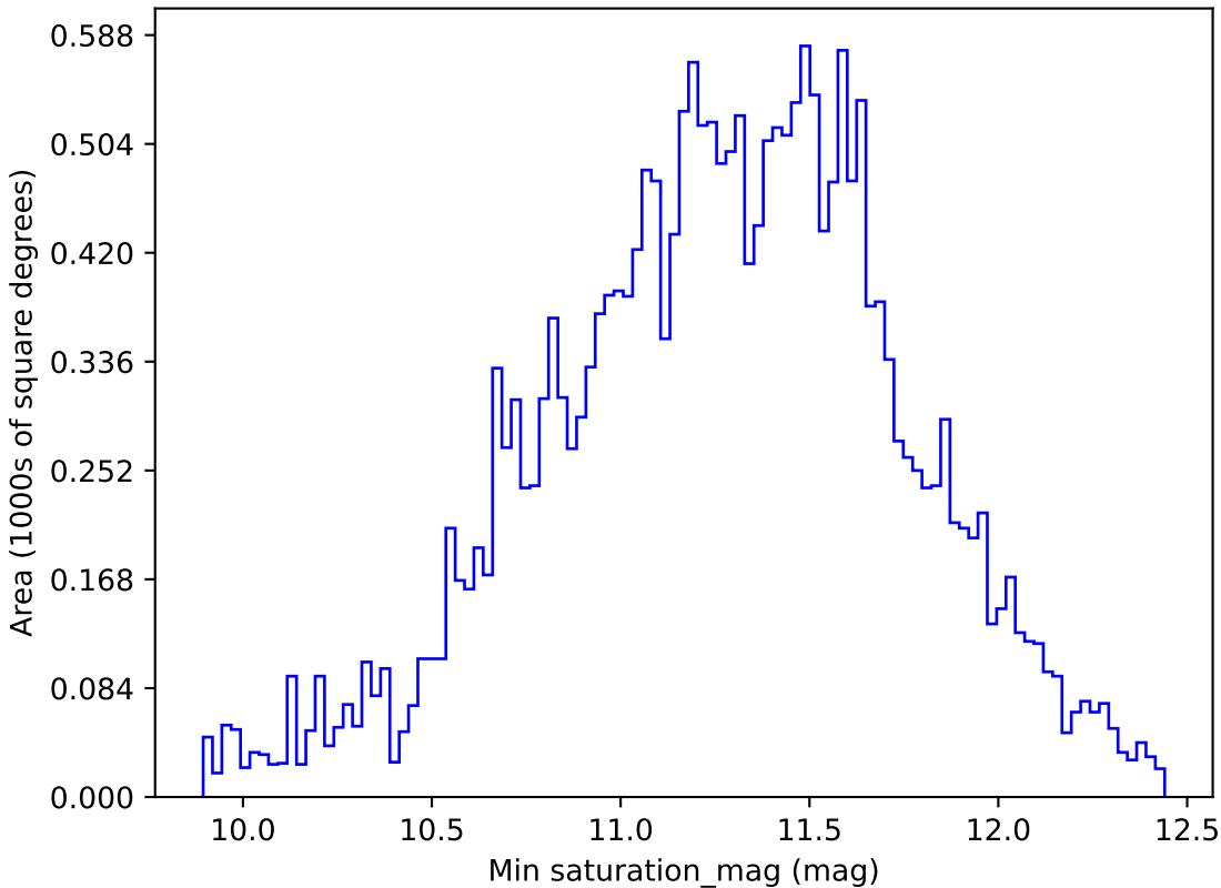
too_elab_r64_d3_gz_v3.4_10yrs All sky y band: Min saturation_mag
