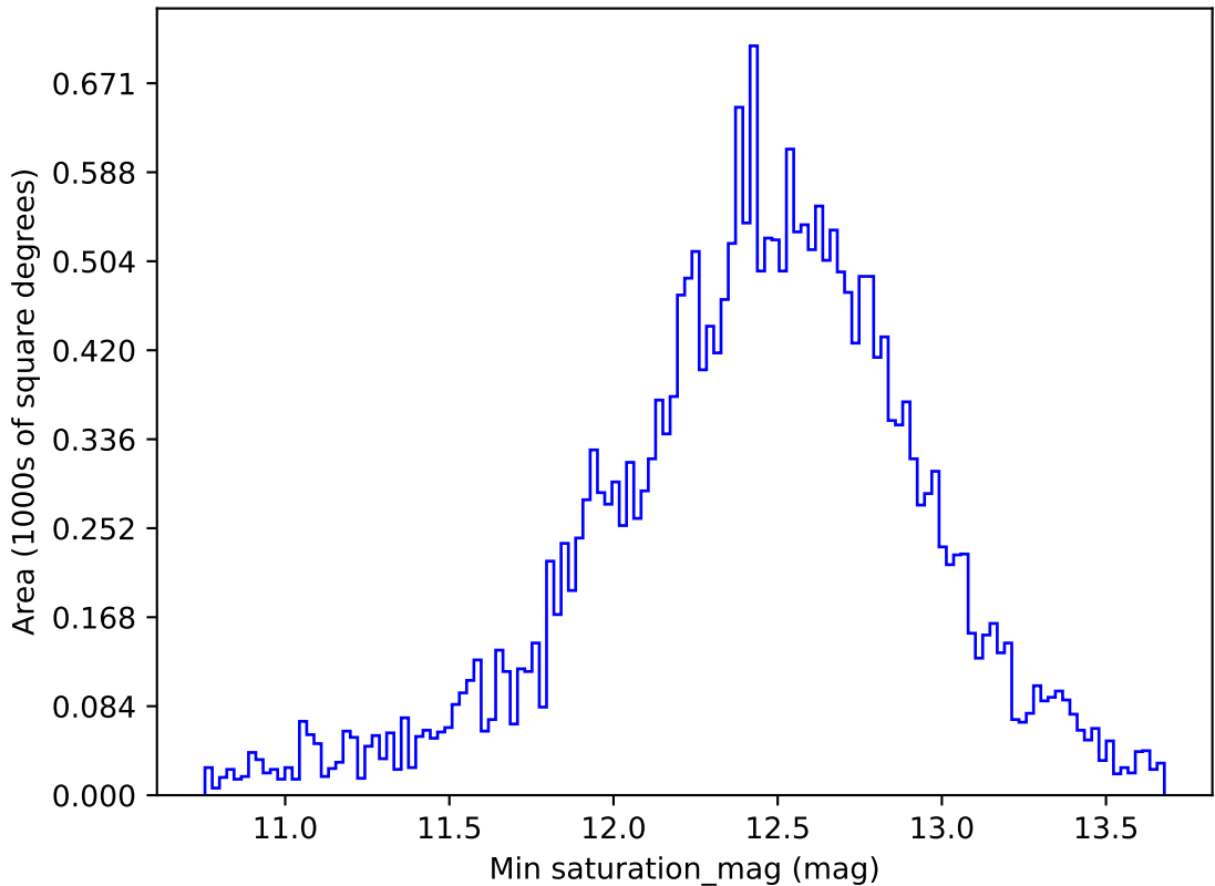
too_elab_r64_d3_gz_v3.4_10yrs All sky i band: Min saturation_mag
