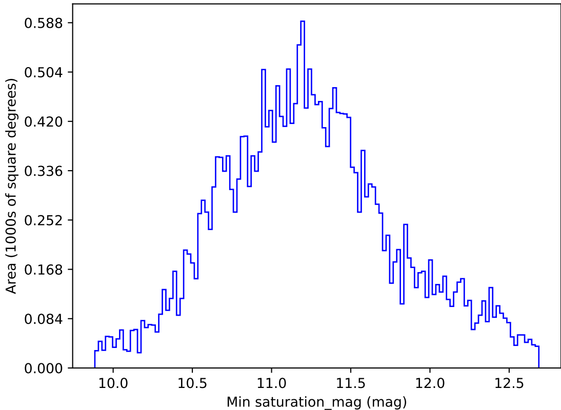
too_elab_r64_d3_gz_v3.4_10yrs All sky all bands: Min saturation_mag
