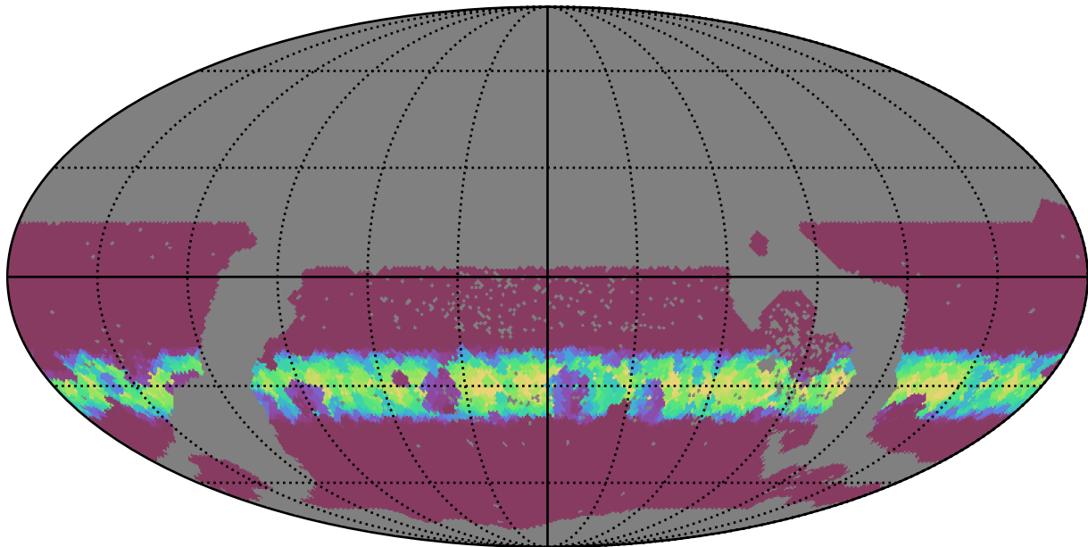
too_elab_r64_d3_gz_v3.4_10yrs WFD all bands: Min normairmass
