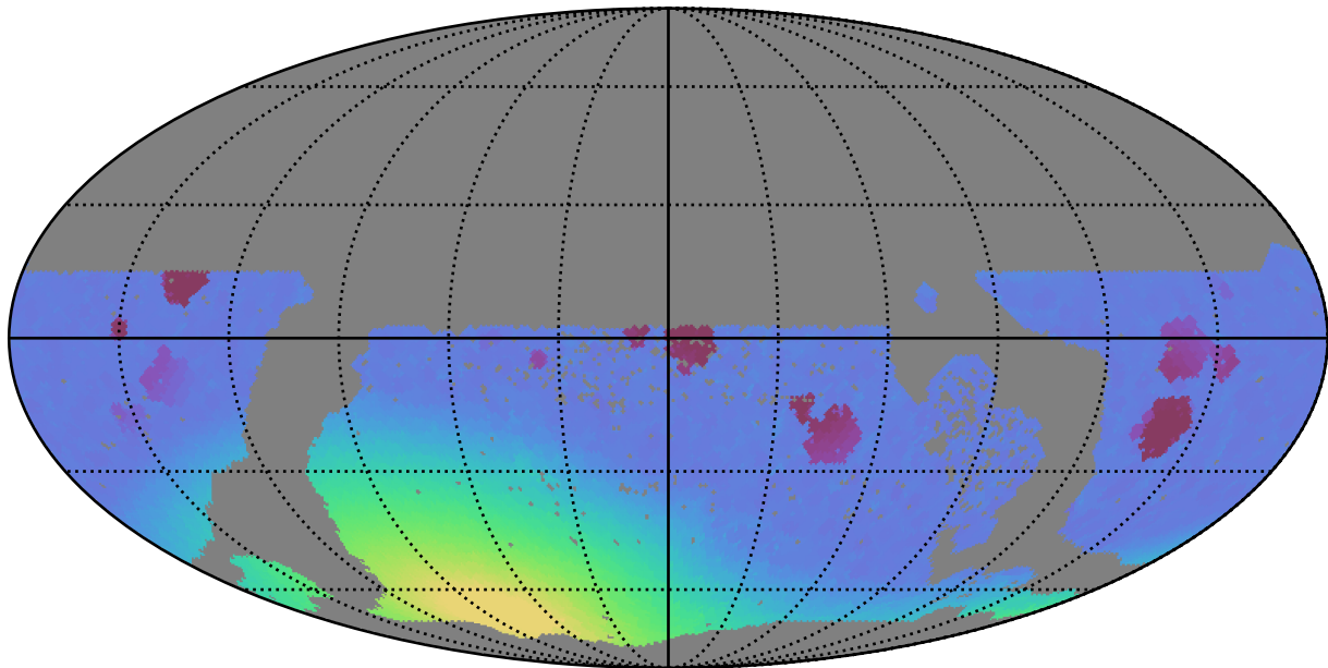
too_elab_r64_d3_gz_v3.4_10yrs WFD z band: Min moonDistance
