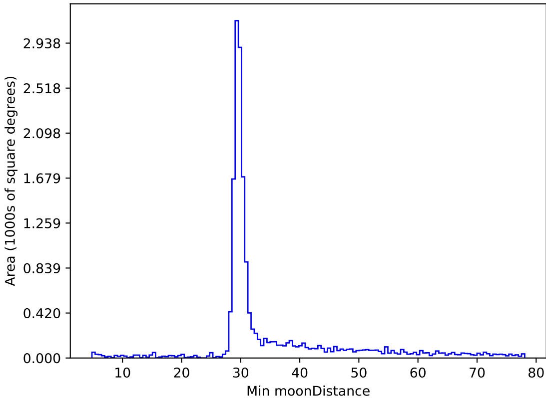
too_elab_r64_d3_gz_v3.4_10yrs WFD z band: Min moonDistance
