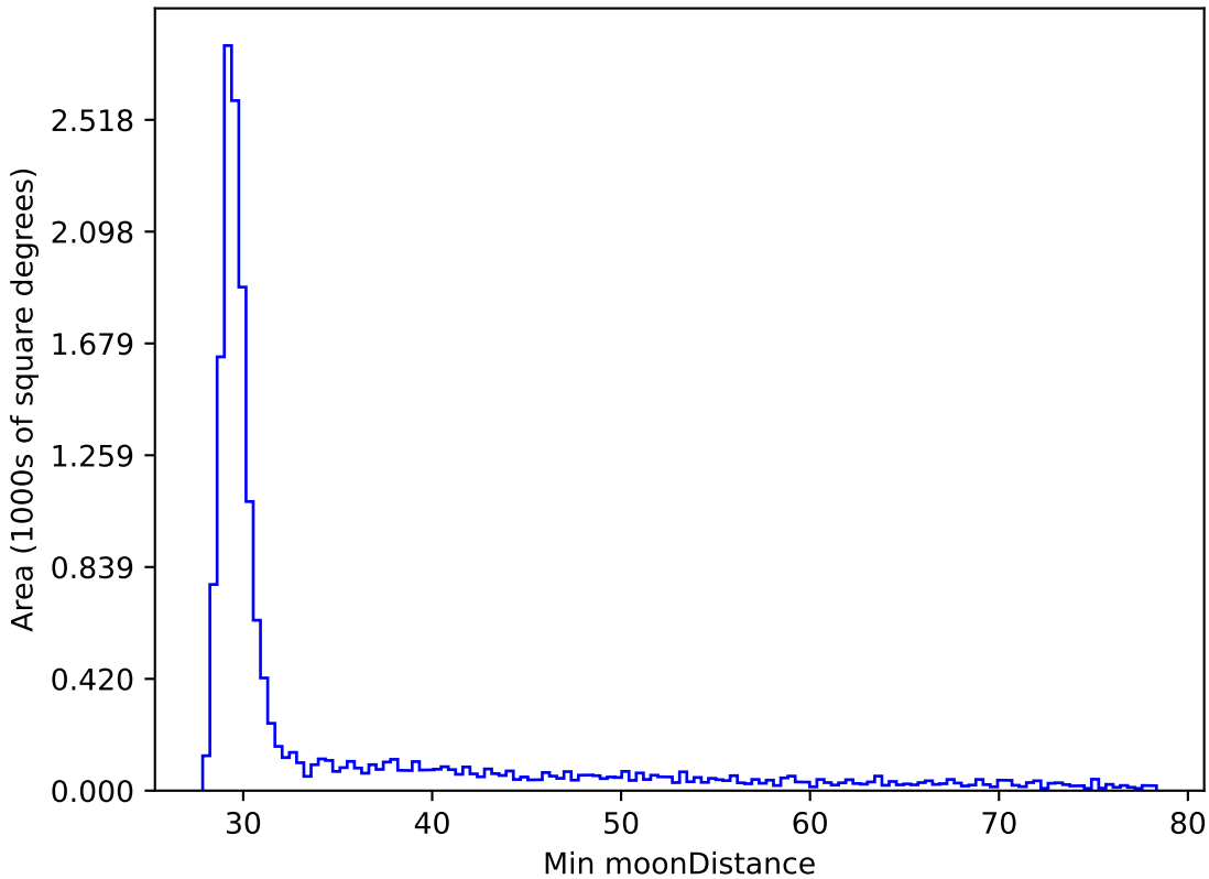
too_elab_r64_d3_gz_v3.4_10yrs WFD y band: Min moonDistance
