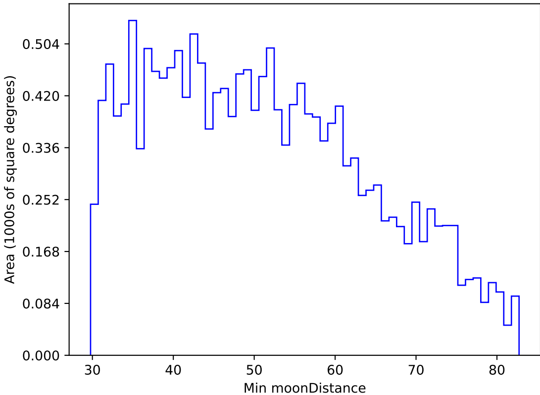
too_elab_r64_d3_gz_v3.4_10yrs WFD u band: Min moonDistance
