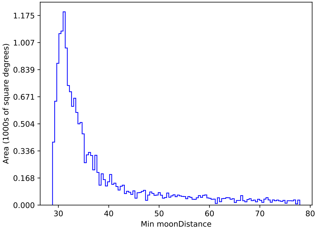
too_elab_r64_d3_gz_v3.4_10yrs WFD r band: Min moonDistance
