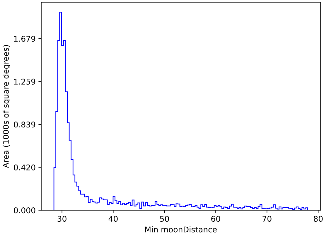
too_elab_r64_d3_gz_v3.4_10yrs WFD i band: Min moonDistance
