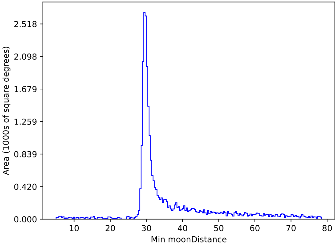
too_elab_r64_d3_gz_v3.4_10yrs All sky z band: Min moonDistance
