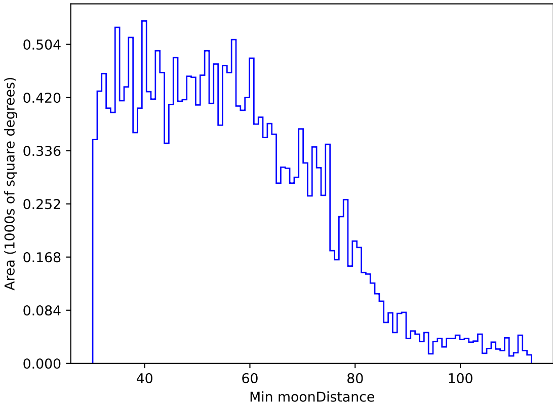
too_elab_r64_d3_gz_v3.4_10yrs All sky u band: Min moonDistance
