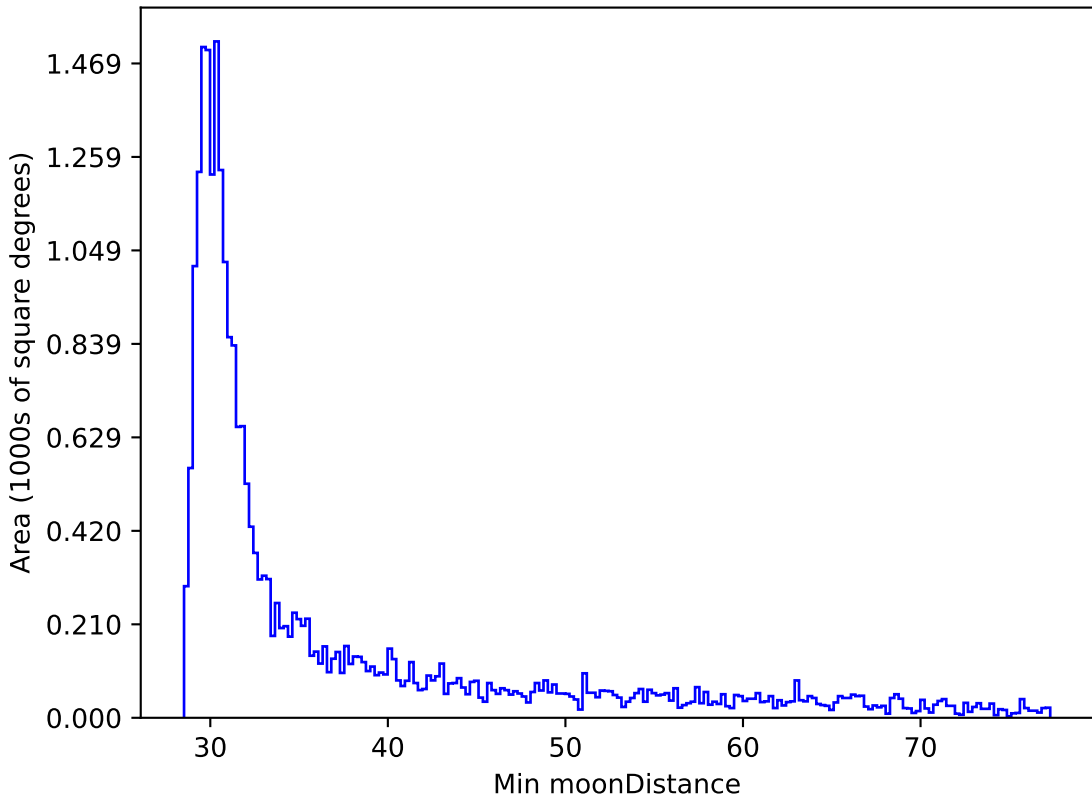
too_elab_r64_d3_gz_v3.4_10yrs All sky i band: Min moonDistance
