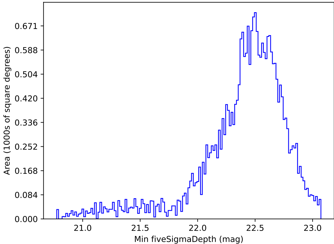
too_elab_r64_d3_gz_v3.4_10yrs Yr 1 z band: Min fiveSigmaDepth
